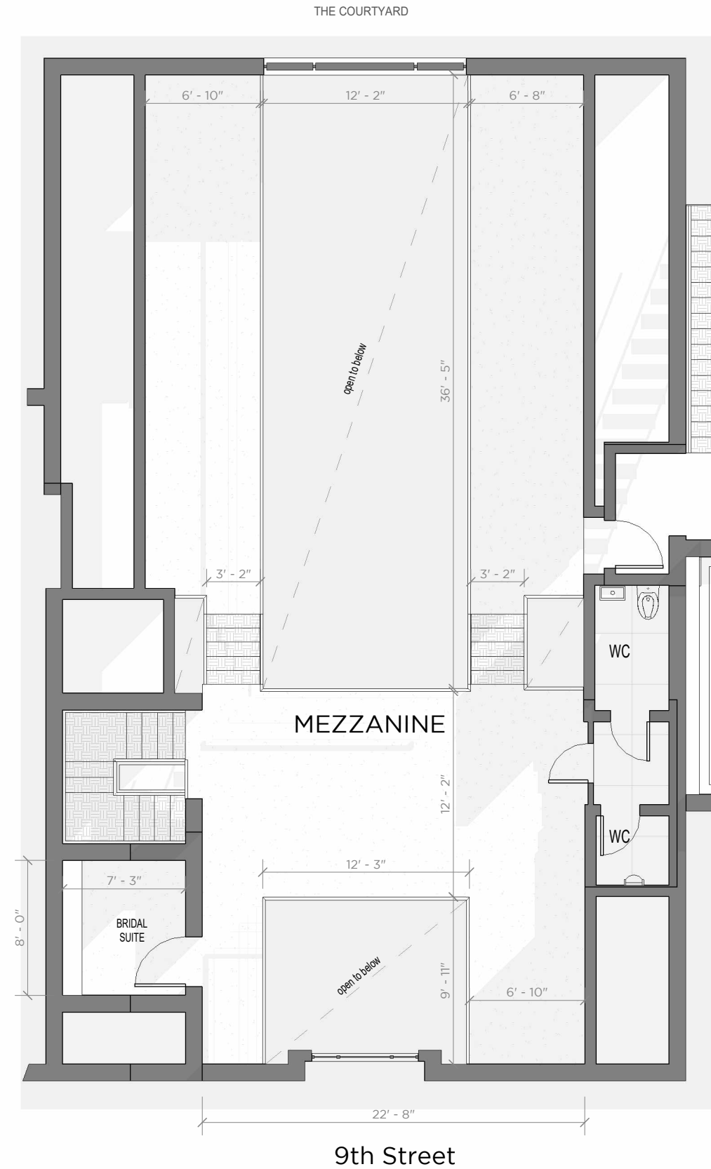
② Main Space Mezzanine 1/8" = 1'-0"
