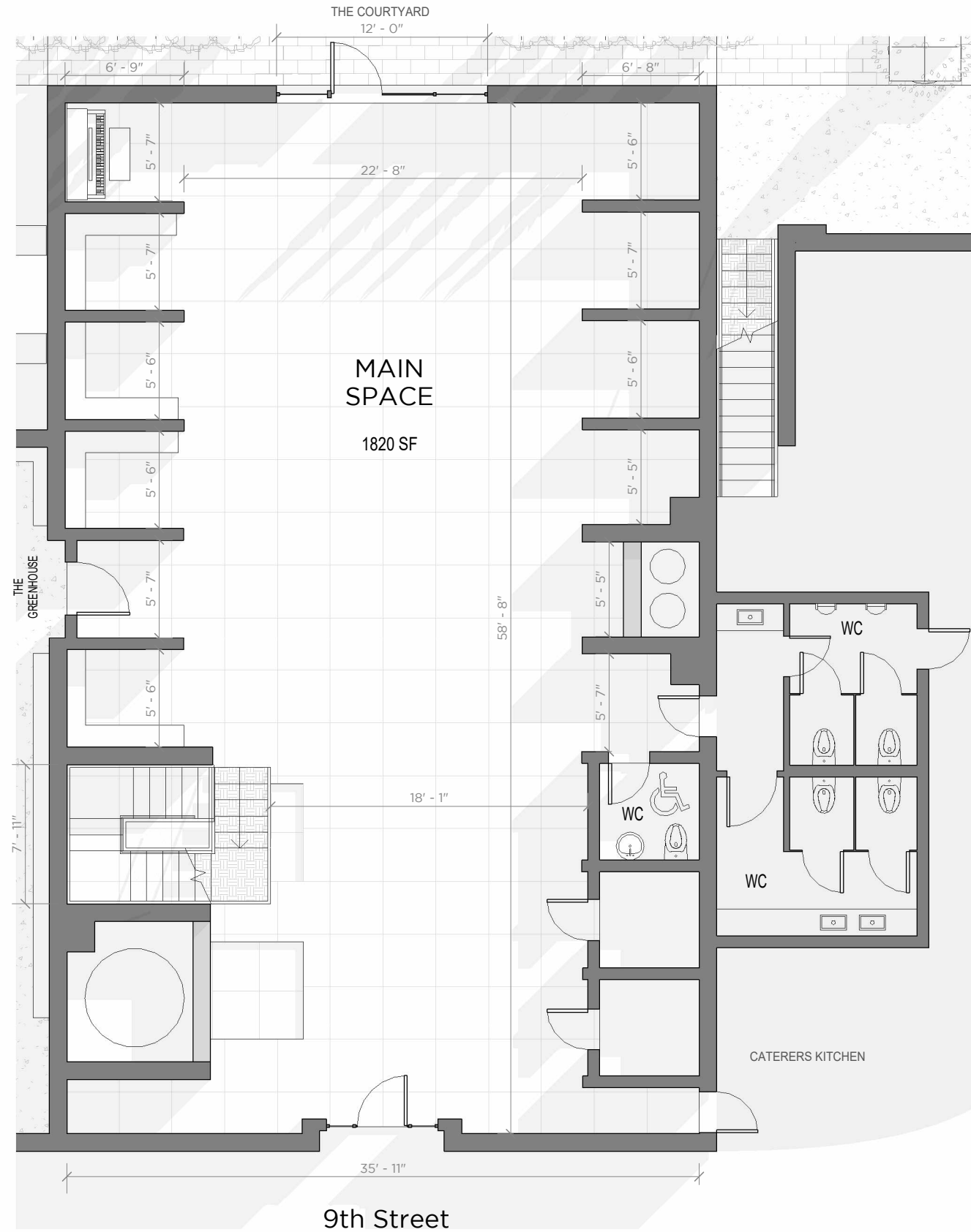
① Main Space Ground 1/8" = 1'-0"
